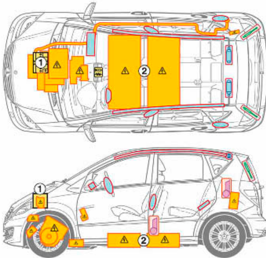
2 High-voltage battery
